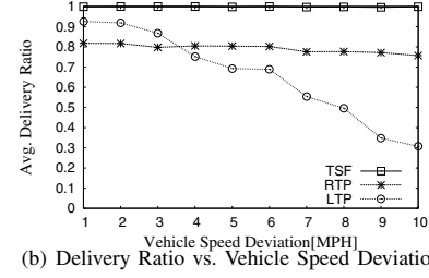
Figure 10. Impact of Vehicle Speed Deviation \sigma_v
