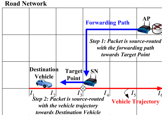
Figure 6. TSF Forwarding Protocol
