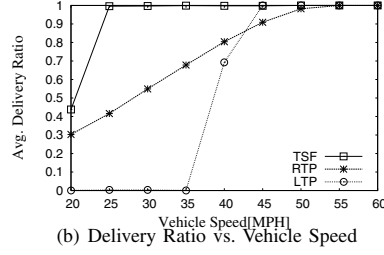
Figure 9. Impact of Vehicle Speed \mu_v
