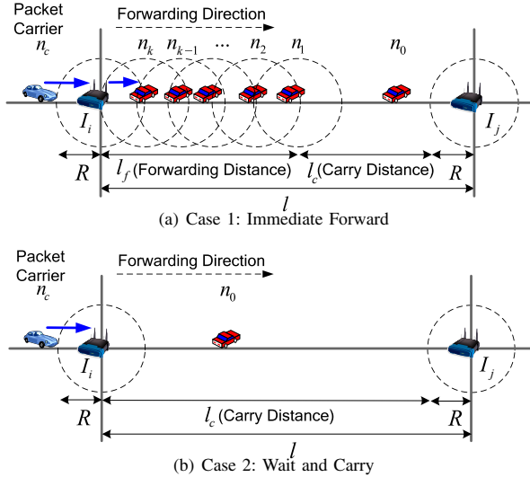
Figure 3. Link Delay Modeling for Road Segment
