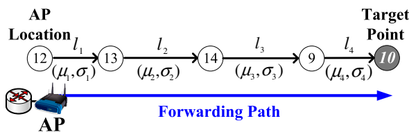
Figure 4. Packet Delay Model from AP to Target Point
