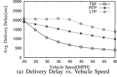
(a) Delivery Delay vs. Vehicle Speed
